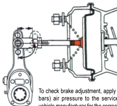
PROPERLY - ADJUSTED BRAKES "ON" - APPLIED
