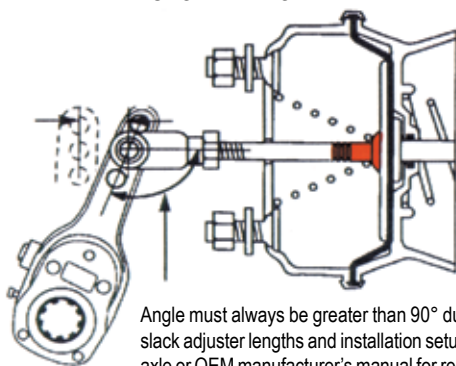
BRAKES "OFF" - NOT APPLIED
